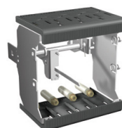
Moving part of a withdrawable circuit-breaker
