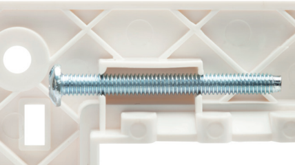
Mounting screws press fitted in back side screw holder to prevent losing of the screws.
